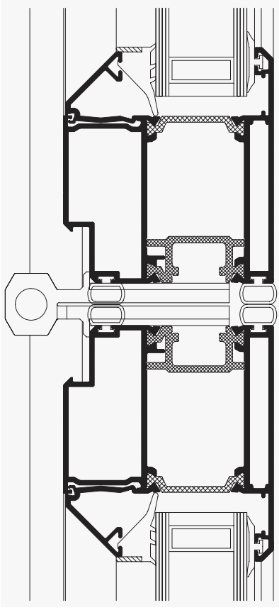
Hinged meeting stiles (open in)
