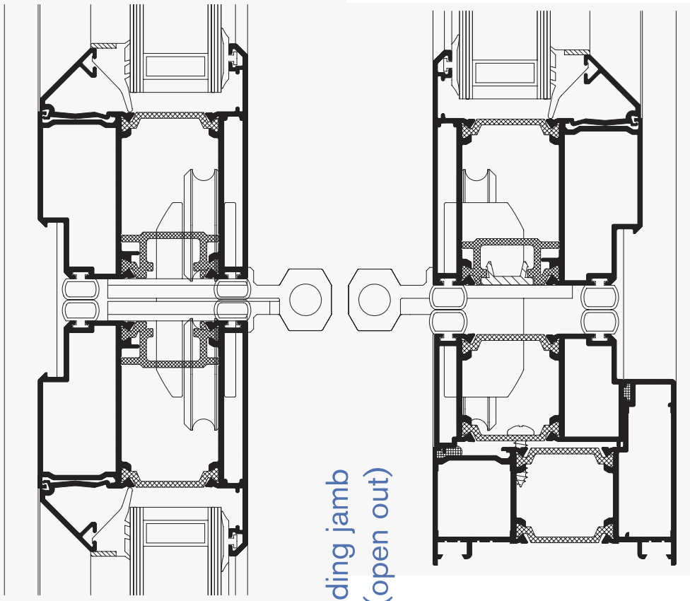
Rolling meeting stiles (open out)
