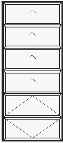
Six pane configuration 651 (6 panes, 5 sliding, 1 swing)
